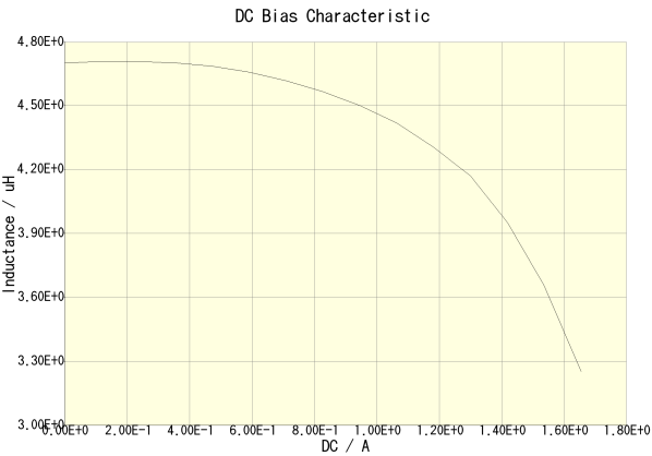
VLS4012ET-4R7M(Amb. Temp. = 20degc)
