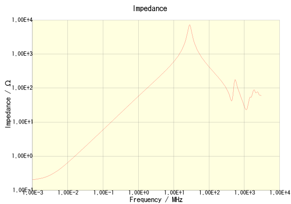
VLS4012ET-100M
