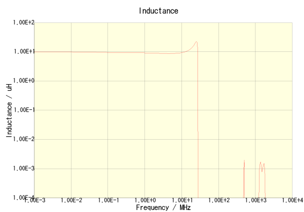
VLS4012ET-100M
