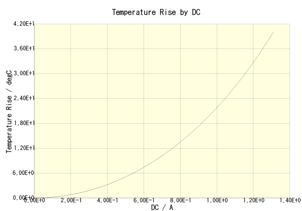
VLS4012ET-100M(Amb. Temp. = 20degc)
