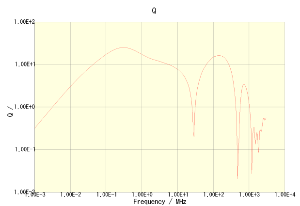
VLS4012ET-100M
