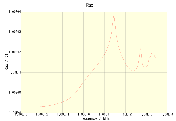
VLS4012ET-100M
