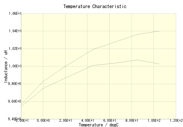
VLS4012ET-100M(DC = 0A)
