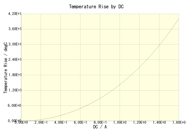
VLS3015ET-4R7M(Amb. Temp. = 20degc)
