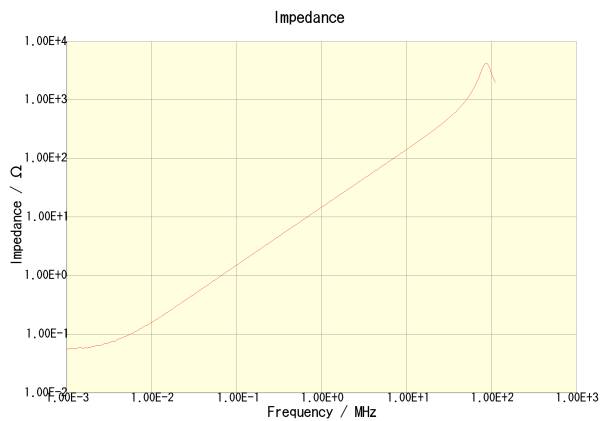
VLCF5020T-2R7N2R2-1
