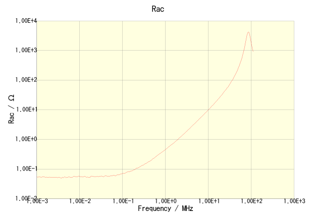
VLCF5020T-2R7N2R2-1
