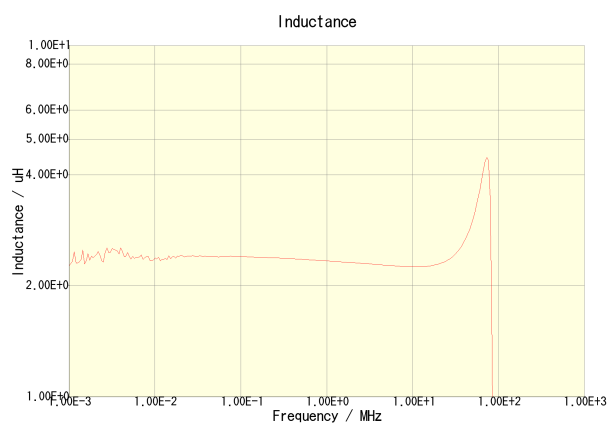
VLCF5020T-2R7N2R2-1
