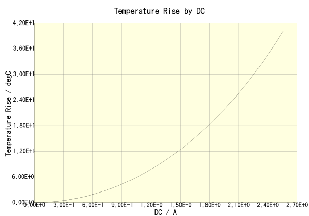
VLCF5020T-2R7N2R2-1(Amb. Temp. = 20degc)
