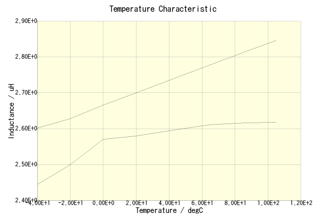
VLCF5020T-2R7N2R2-1(DC = 0A)
