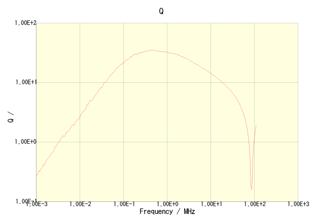
VLCF5020T-2R7N2R2-1
