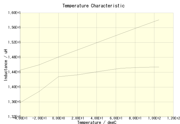
VLCF5020T-150MR90-1(DC = 0A)
