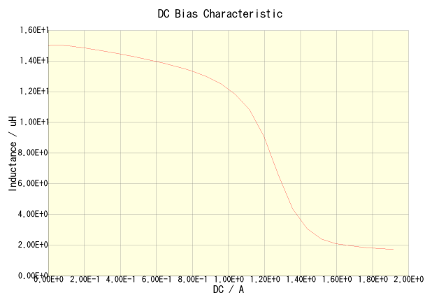
VLCF5020T-150MR90-1(Amb. Temp. = 20degC)
