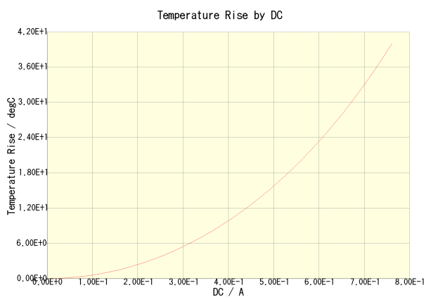
VLCF4020T-270MR48(Amb. Temp. = 20degC)
