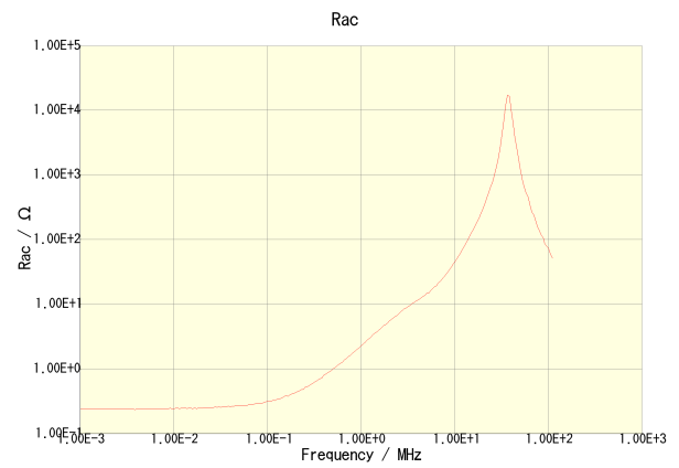
VLCF4018T-150MR59-2
