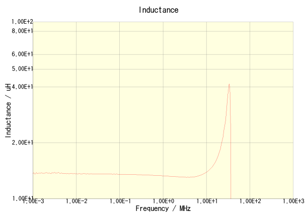
VLCF4018T-150MR59-2
