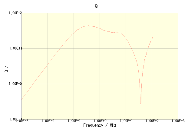
VLCF4018T-150MR59-2
