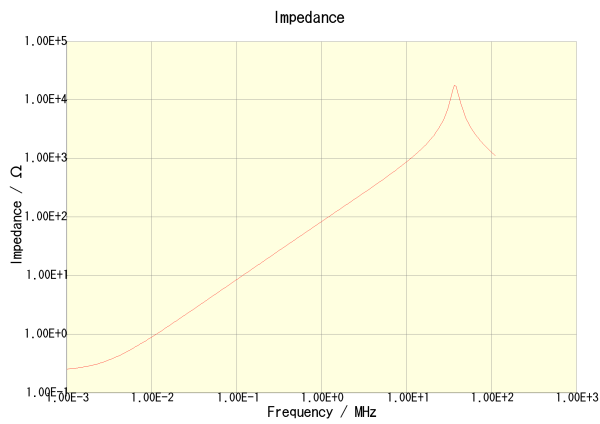
VLCF4018T-150MR59-2
