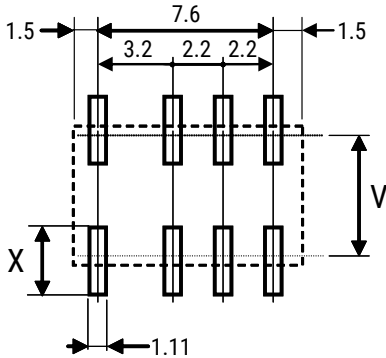
UB2 Series (top view)
