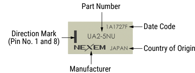
UA2 – Top View
