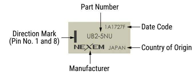
UB2 – Top View
