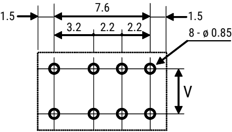
UA2 Series (bottom view)
