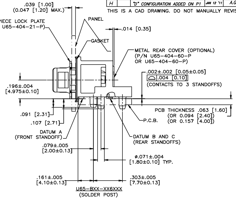
DIMENSION TABLE:
