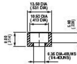
U840 (for cap U480)
