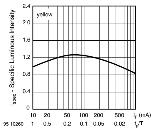
Fig. 12 - Relative Luminous Intensity vs. Forward Current / Duty Cycle
