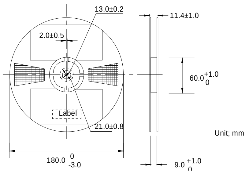
Carrier Tape
