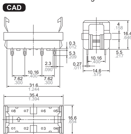
Terminal socket for soldering
