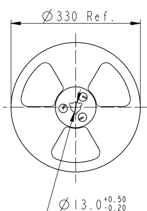
Reel For Carrier Tape
