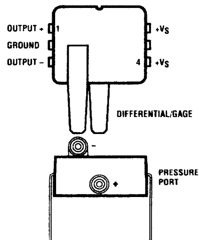
"D4" DIP PACKAGE
