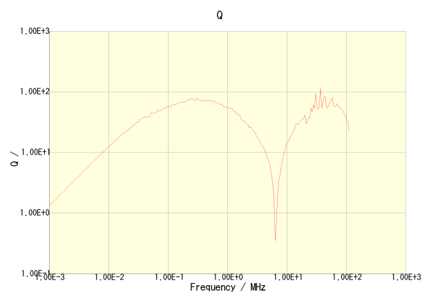
SLF7032T-221MR29-2PF
