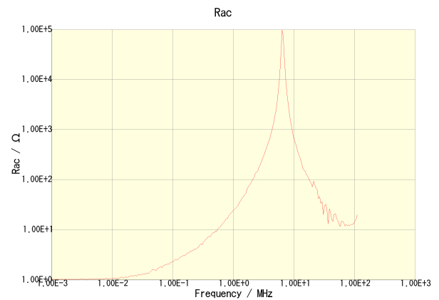
SLF7032T-221MR29-2PF
