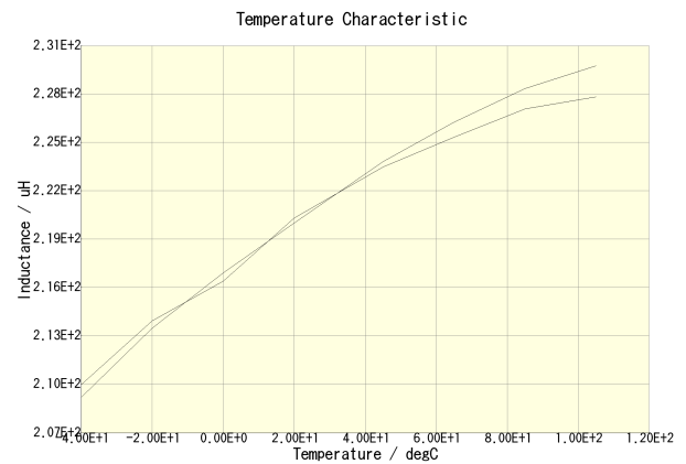
SLF7032T-221MR29-2PF(DC = 0A) SLF7032T-221MR29-2PF(DC = 0.145A)
