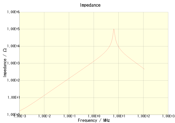
SLF7032T-221MR29-2PF
