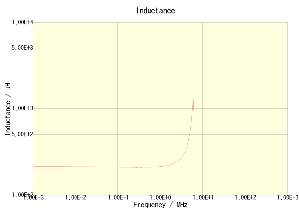
SLF7032T-221MR29-2PF
