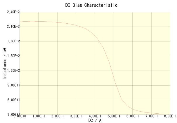
SLF7032T-221MR29-2PF(Amb. Temp. = 20degc)
