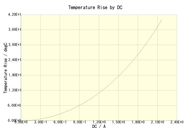
SLF7032T-150M1R1-2PF(Amb. Temp. = 20degc)
