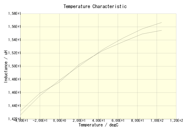
SLF7032T-150M1R1-2PF(DC = 0A) SLF7032T-150M1R1-2PF(DC = 0.55A)
