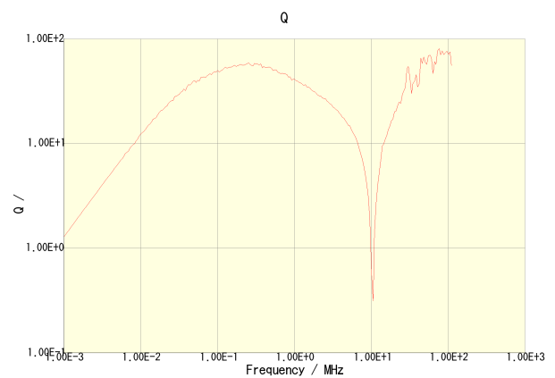
SLF7032T-101MR45-2PF
