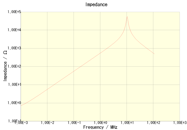
SLF7032T-101MR45-2PF
