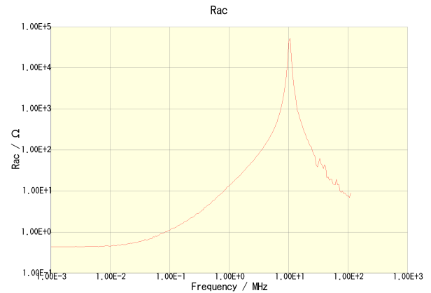
SLF7032T-101MR45-2PF
