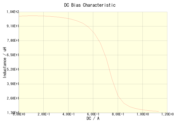
SLF7032T-101MR45-2PF(Amb. Temp. = 20degc)
