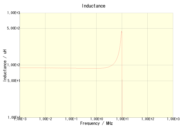
SLF7032T-101MR45-2PF
