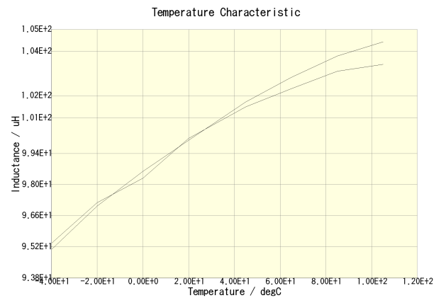
SLF7032T-101MR45-2PF(DC = 0A) SLF7032T-101MR45-2PF(DC = 0.225A)
