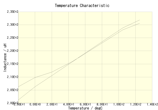
SLF12575T-221M1R3-H(DC = 0A) SLF12575T-221M1R3-H(DC = 0.65A)
