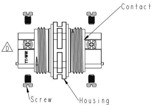
⑥ Connector
