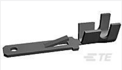
TE Part #160457-2 FF 250 TAB 18-14AWG TPPB
