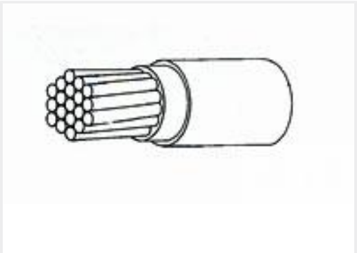
TE Part #218208-002 22759/34-16-9
