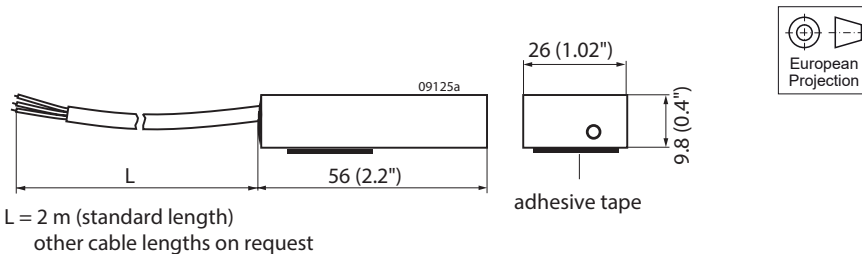
Fig. 6 S-KSMH temperature sensor.
