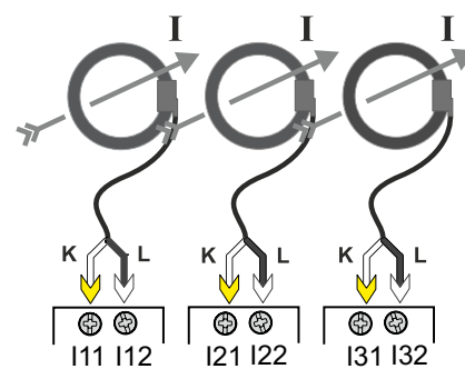
Fig. 3 Connection with EM50, K=white (yellow ferrule), L=black (white ferrule)
