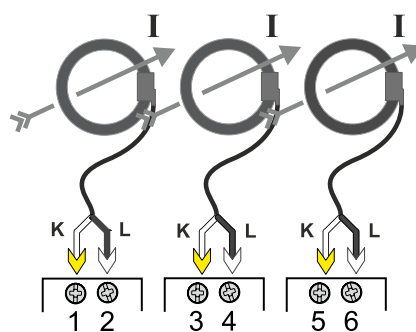
Fig. 2 Connection with EM210, K=white (yellow ferrule), L=black (white ferrule)
