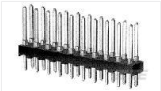
TE Part #87227-2 04 MODII HDR DRST UNSHRD .100
