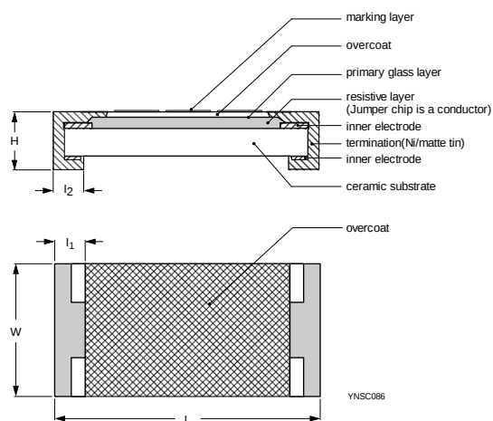
Fig. 9 Chip resistor outlines
