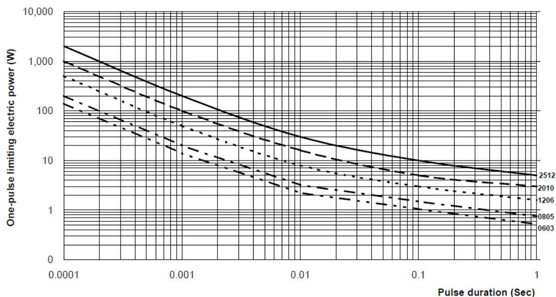
Fig. 14 Maximum permissible peak pulse power as a function of pulse duration
