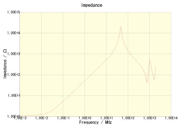
NLV32T-8R2J-PF
