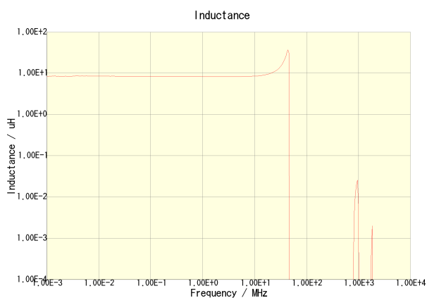
NLV32T-8R2J-PF
