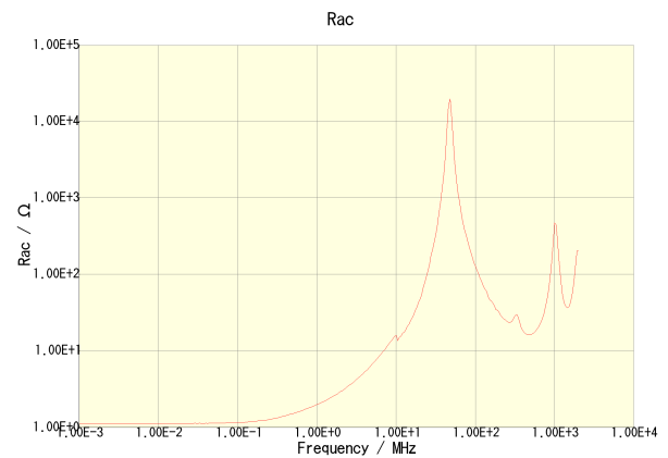
NLV32T-8R2J-PF
