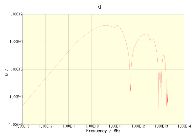
NLV32T-8R2J-PF
