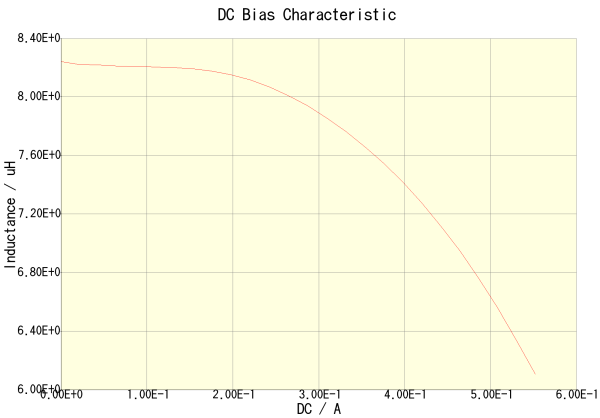
NLV32T-8R2J-PF(Amb. Temp. = 20degc)
