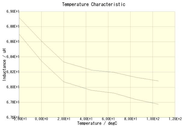
NLV32T-680J-PF(DC = 0A)
