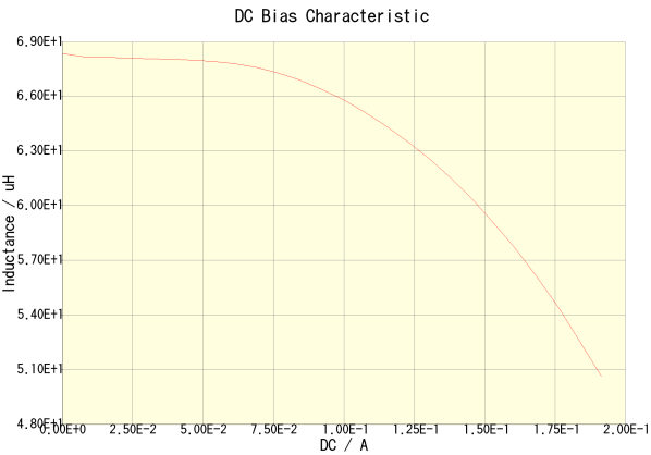
NLV32T-680J-PF(Amb. Temp. = 20degc)
