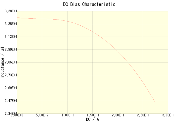
NLV32T-330J-PF(Amb. Temp. = 20degc)
