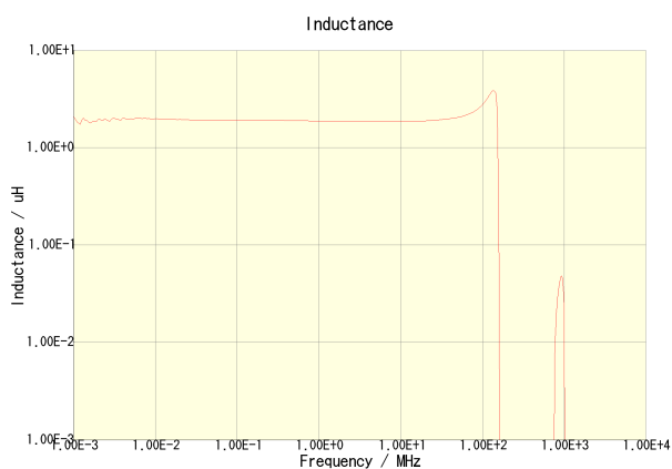
NLV32T-1R8J-PF
