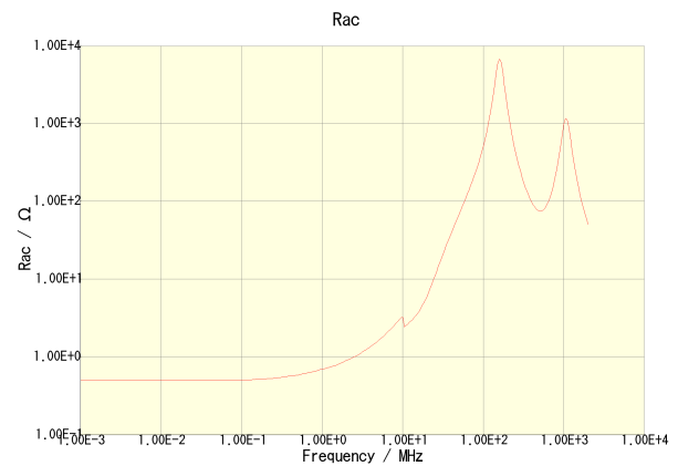
NLV32T-1R8J-PF
