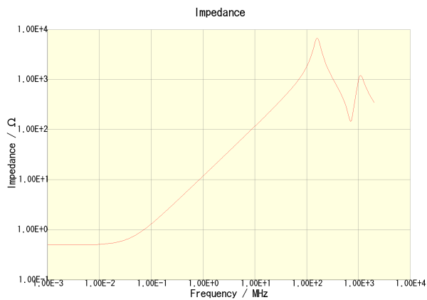
NLV32T-1R8J-PF
