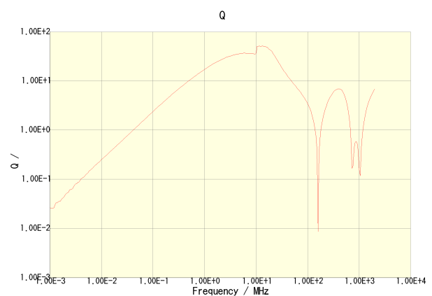
NLV32T-1R8J-PF
