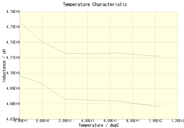
NLV25T-4R7J-PF(DC = 0A)
