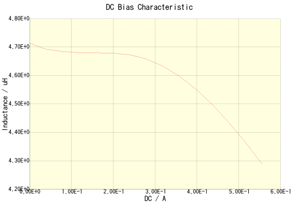
NLV25T-4R7J-PF(Amb. Temp. = 20degc)
