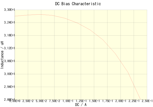
NLV25T-330J-PF(Amb. Temp. = 20degc)
