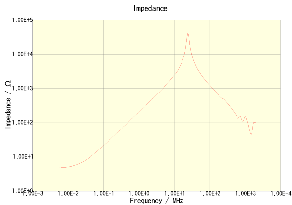
NLV25T-330J-PF
