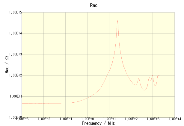
NLV25T-330J-PF
