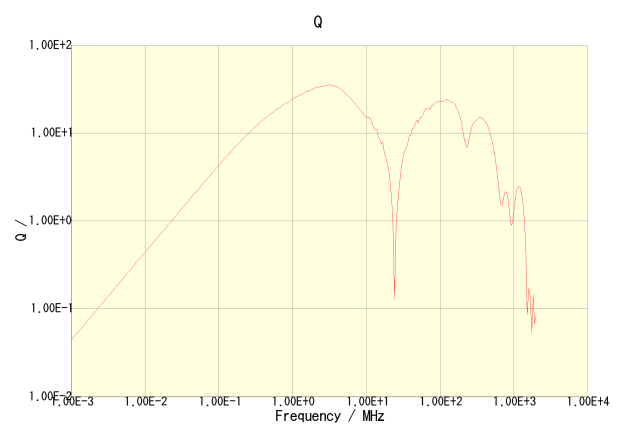
NLV25T-330J-PF
