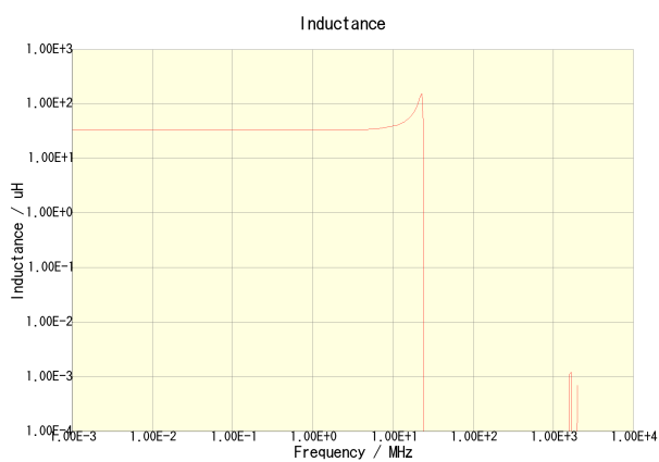
NLV25T-330J-PF
