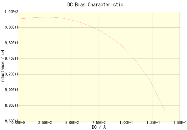
NLV25T-101J-PF(Amb. Temp. = 20degc)
