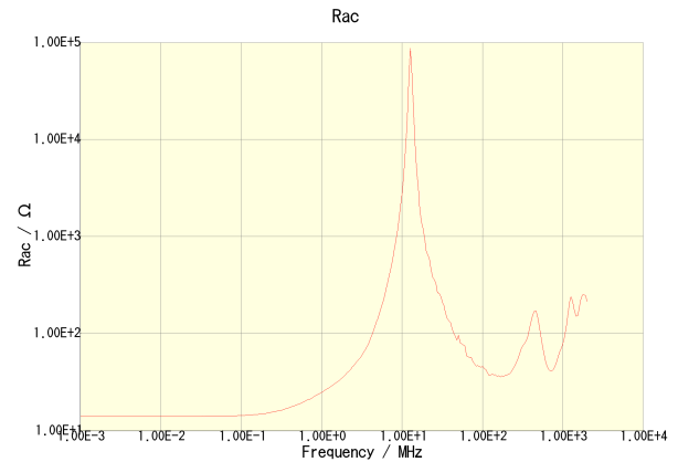
NLV25T-101J-PF
