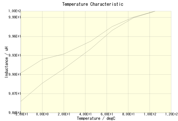
NLV25T-101J-PF(DC = 0A)
