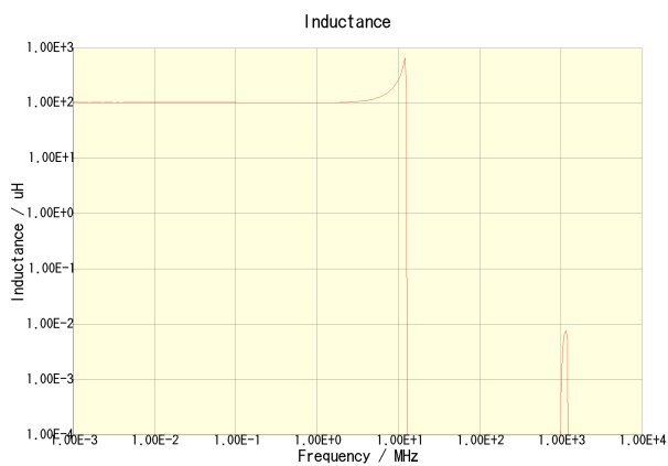
NLV25T-101J-PF
