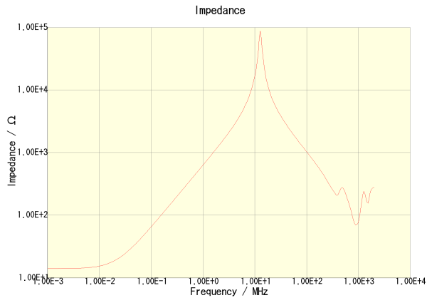
NLV25T-101J-PF
