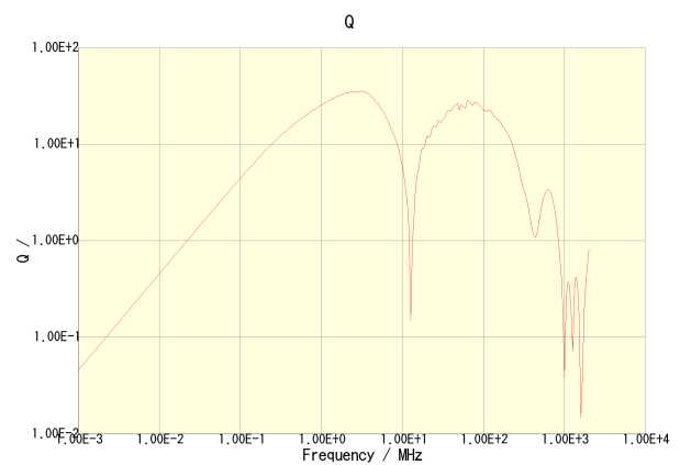
NLV25T-101J-PF
