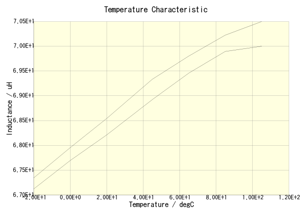
NLCV32T-680K-PF(DC = 0A)
