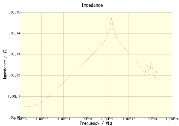
NLCV32T-680K-PF
