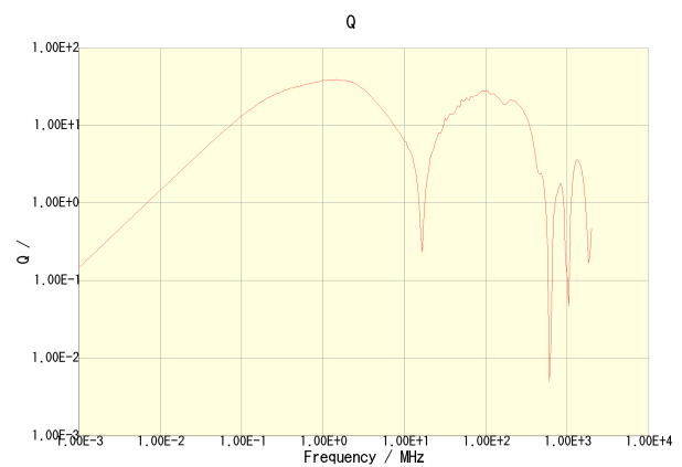
NLCV32T-680K-PF
