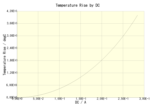
NLCV32T-680K-PF(Amb. Temp. = 20degc)
