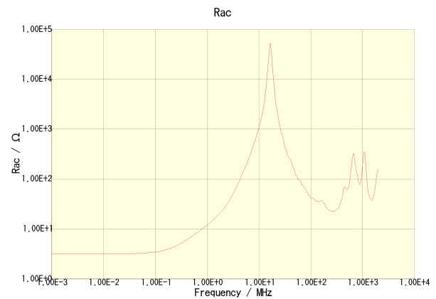
NLCV32T-680K-PF
