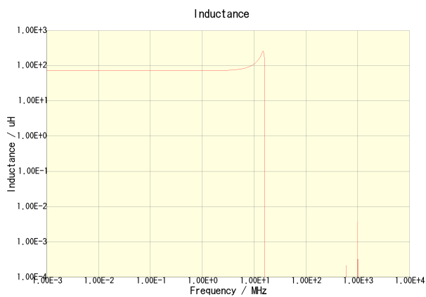
NLCV32T-680K-PF
