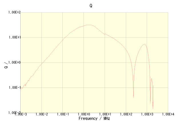
NLCV32T-1R0M-PF
