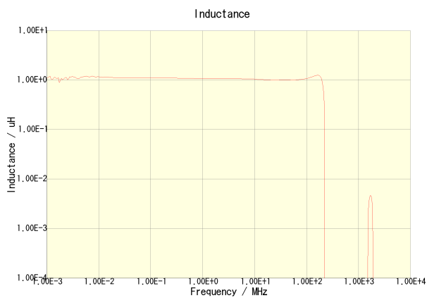
NLCV32T-1R0M-PF
