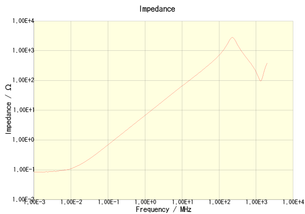
NLCV32T-1R0M-PF
