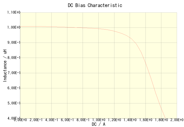
NLCV32T-1R0M-PF(Amb. Temp. = 20degC)
