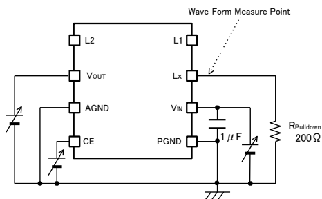
< Circuit No.⑤ >
