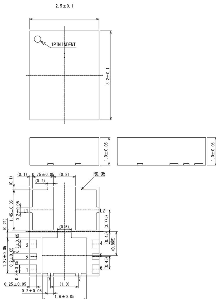
●Reference Pattern Layout (unit: mm)
