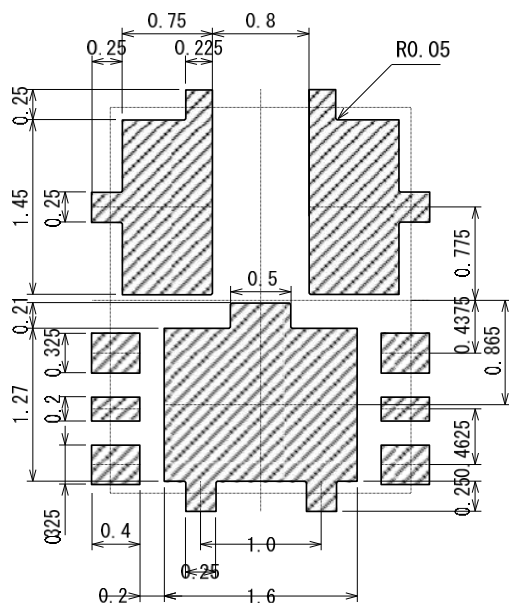
●Reference Pattern Layout (unit: mm)
