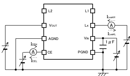
< Circuit No.⑦ >
