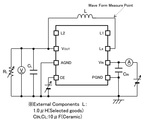
< Circuit No.① >
