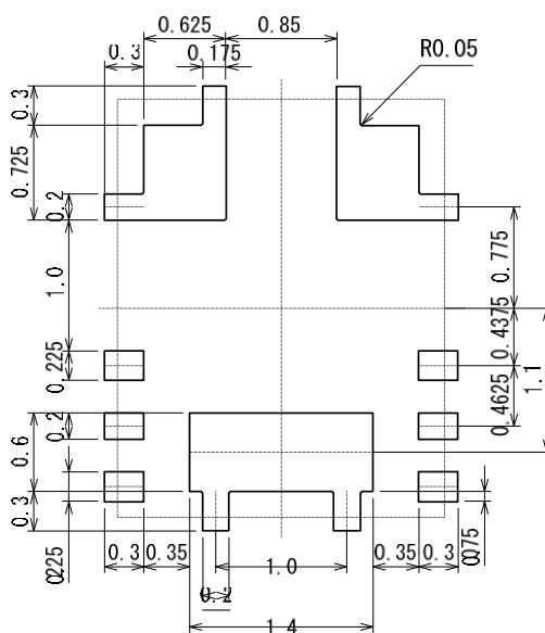
●Reference Metal Mask Design (unit: mm)
