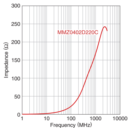
MMZ0402D series
