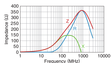
MMZ0402EUC151CTF0W
