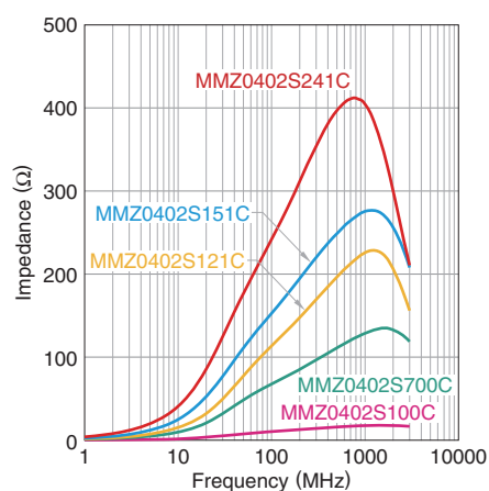
MMZ0402S series
