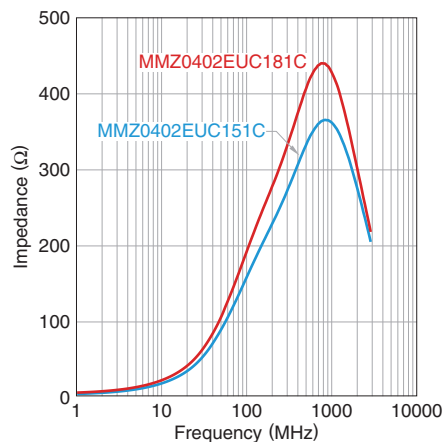
MMZ0402EUC series
