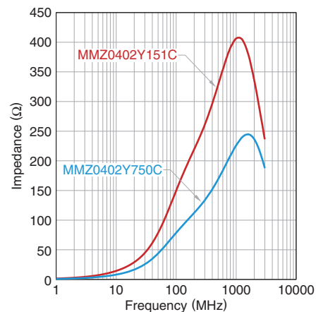
MMZ0402Y series
