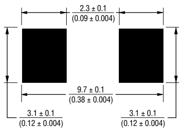
Recommended Pad Layout MF-SMHT136
