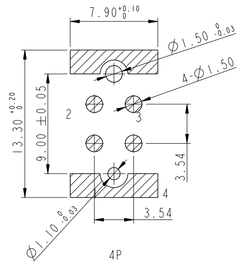
PCB Layout
