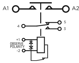
Circuit Configuration 1
