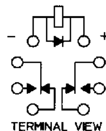
TERMINAL VIEW
