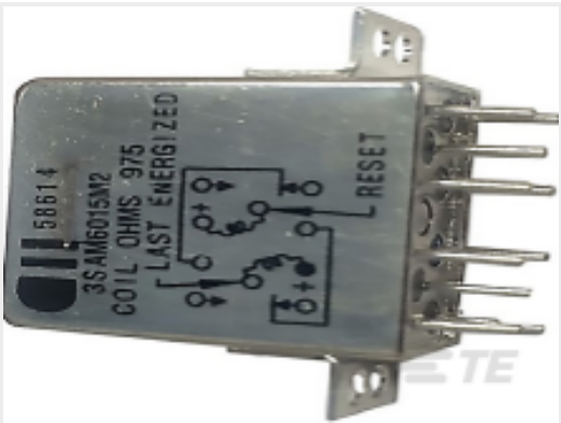
TE Part # 3-1617514-4 3SAT1331A2=M5757/13-114
