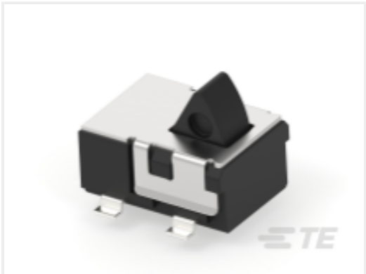
TE Part # 2331394-1 DET SW4.7X3.5X2.25 GW VERT. NOH AG RL
