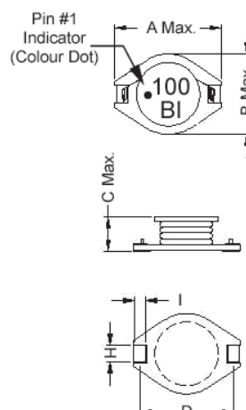
Figure 3 (Case Size: 20 & 50)
