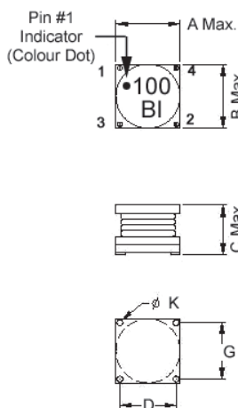
Figure 2 (Case Size: 40)
