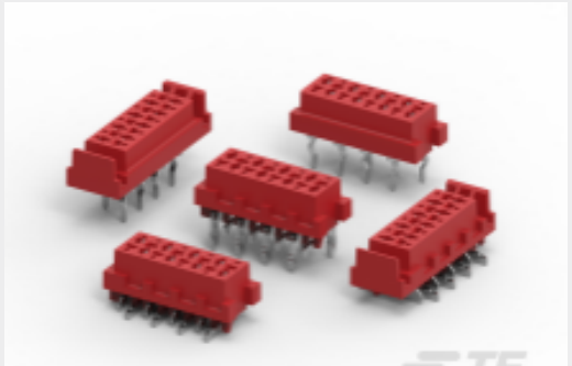
TE Part #CAT-M5833-F3492A Female-on-Board Connector, Top Entry
