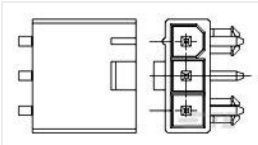
TE Part #2029154-4 4P R/A HDR VAL-U-LOK GW W/P
