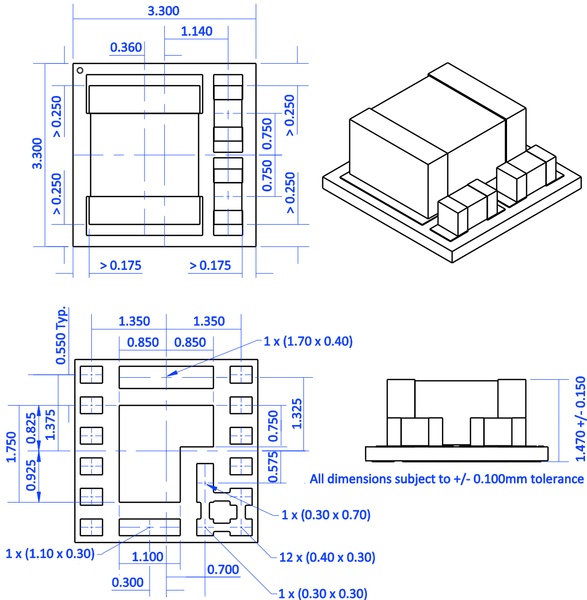
Figure 31 Dimensioned drawings
