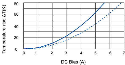
[ ETQP4M4R7YFP ]
