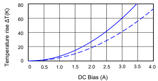
[ ETQP4M100YFP ]
