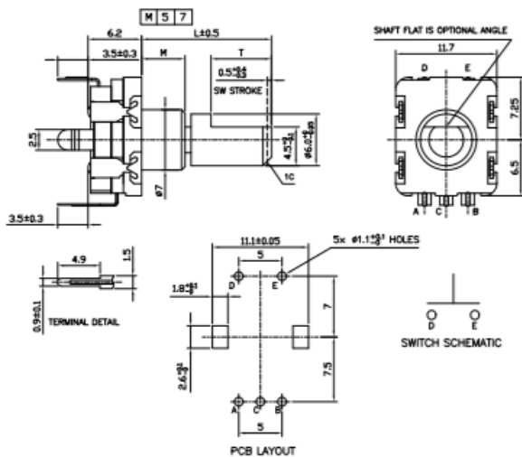
(Top Adjust, with Switch, Plain Bushing)
